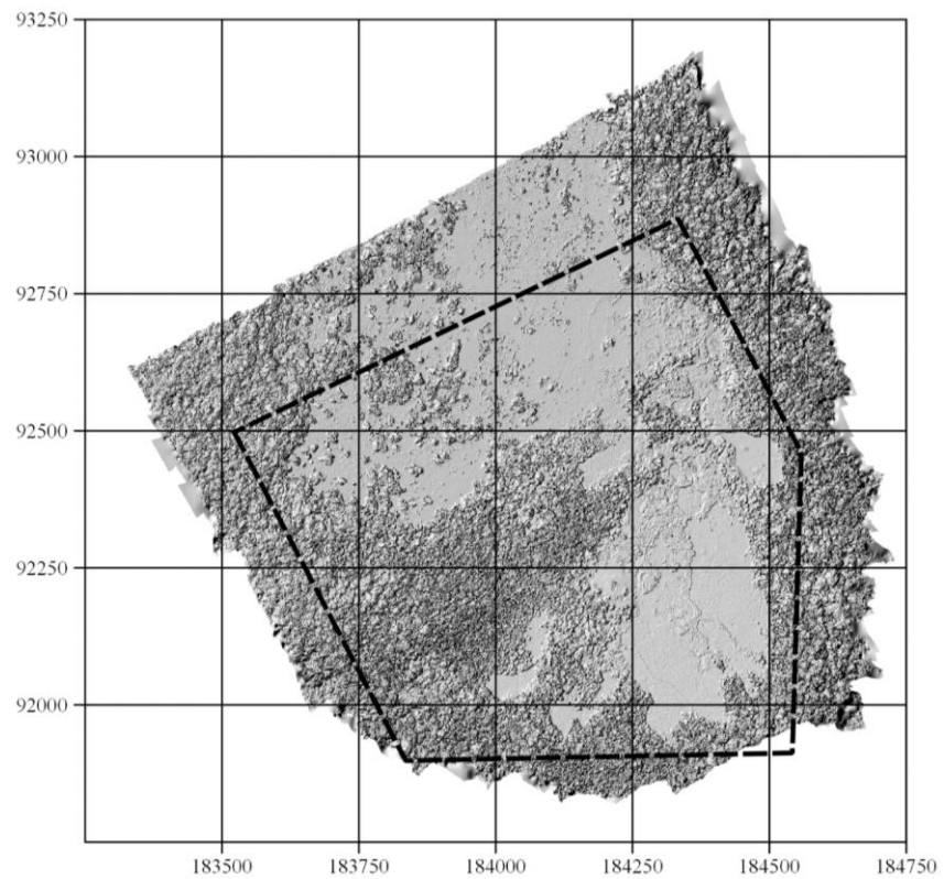
Figure 7: Digital surface model (DSM). Map Datum WGS84. Note: Black dash line shows survey target area.
