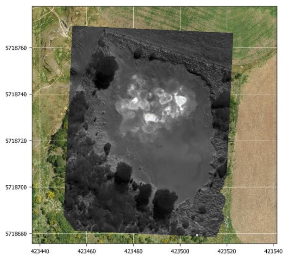
Figure 7: Thermal orthomosaic. Lighter shading indicates higher temperature.
